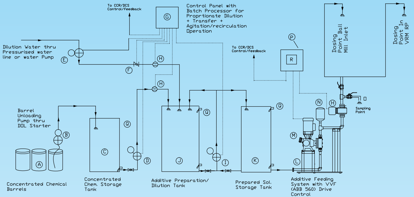
CCR CONTROLLED AUTOMATIC ADDITIVE PREPARATION , MILL TPH LINKED DOSING , FLOW MONITORING AND TOTALISING SYSTEM
